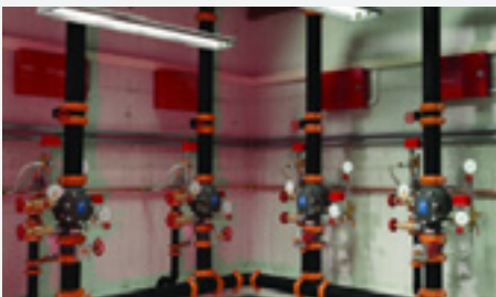
Firefighting System
